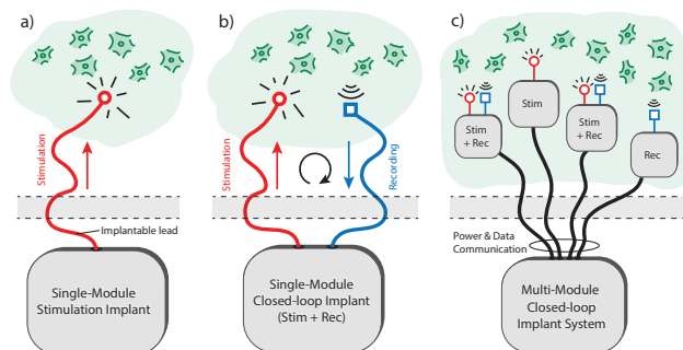
Fig. 1. Comparison between different IMD generations: (a) single-module pace-making stimulation implant, (b) single-module closed-loop stimulation and recording implant, and (3) multi-module closed-loop implant system.
